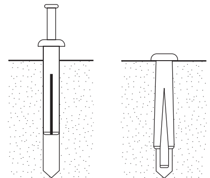
Insert anchor into the pre-drilled hole. Lightly tap on the hammer pin expanding the anchor body until the head is flush with the surface.
