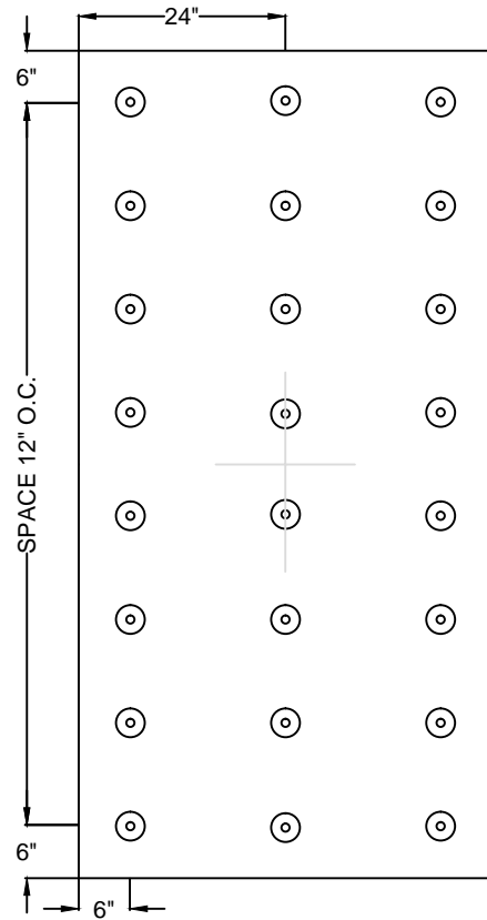
PERIMETER: 24 FASTNERS PER BOARD
