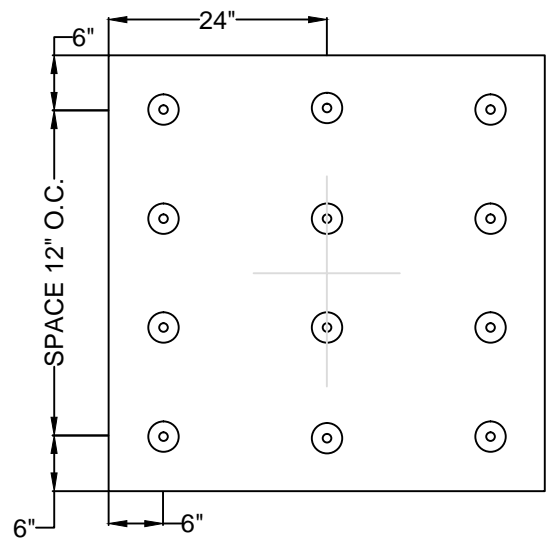
PERIMETER: 12 FASTNERS PER BOARD
