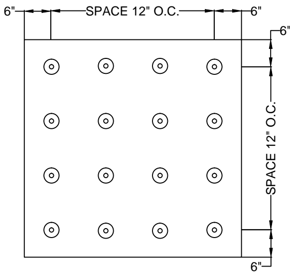
CORNER: 16 FASTNERS PER BOARD
