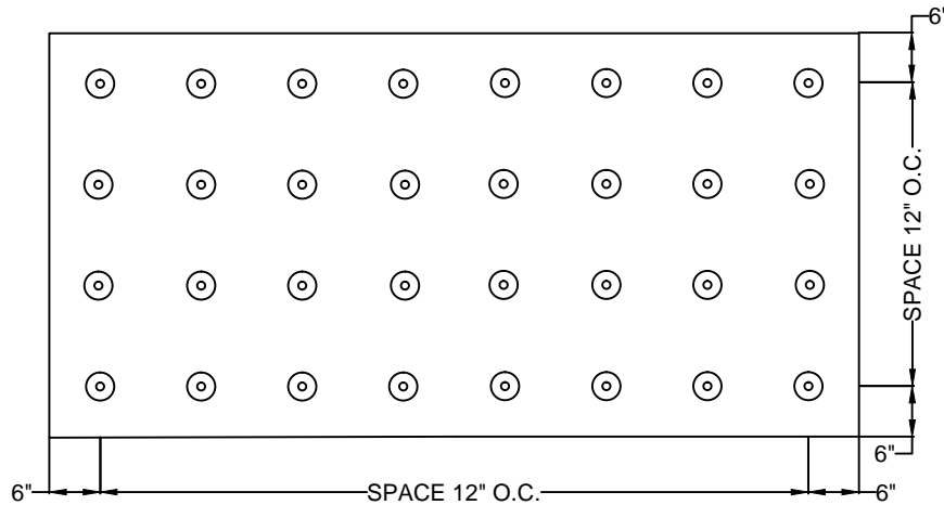
CORNER: 32 FASTNERS PER BOARD
