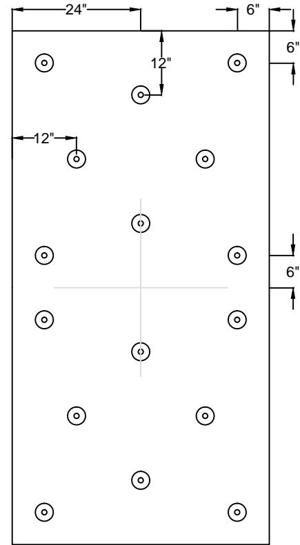
PERIMETER: 16 FASTNERS PER BOARD
